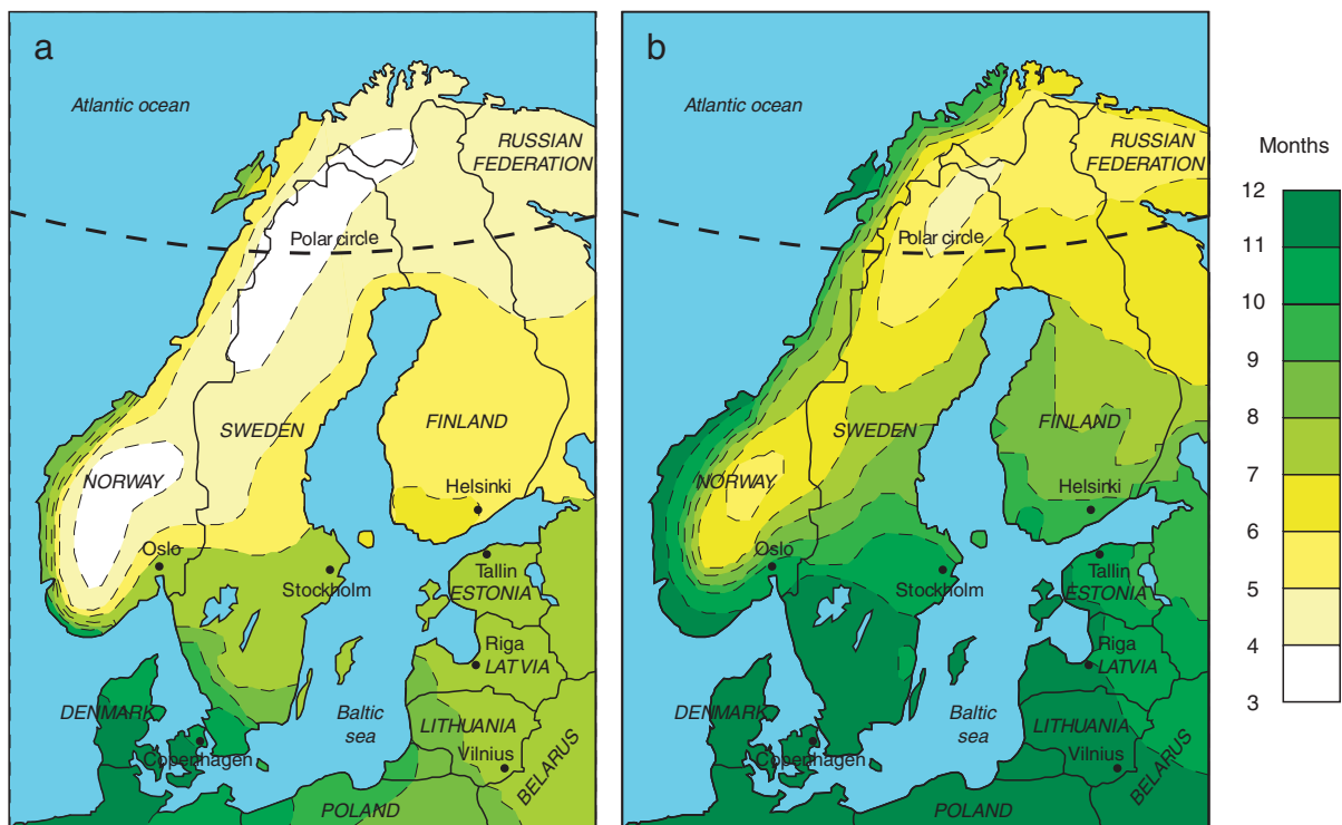
Fig. 1 Number of months with a mean 24-hour temperature above +5^{\circ}\text{C} for the years 1961–1990 (a) and 2070–2100 (b) visualizing an annual move of the zones northward of 5 to 8 km. The map is based on predictions made by SweClim (Rummukainen et al. 2004; Kjellström et al. 2005). Despite this rapid change, temperature sums, extreme long-day conditions
